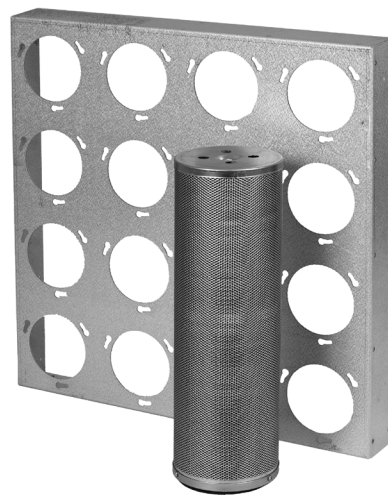
The image shows an activated carbon filter cartridge and a mounting frame designed for 16 filter cartridges. The filter cartridges are filled with 2.5 kg of activated carbon. The cartridges are easily mounted in the frame with a bayonet mount.
